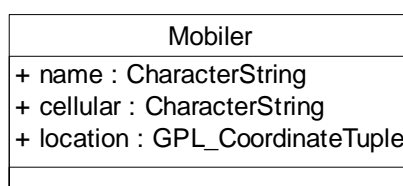
Figure F.2 — Example of UML class diagram of Tracking in Location Based Services (LBS) applications
