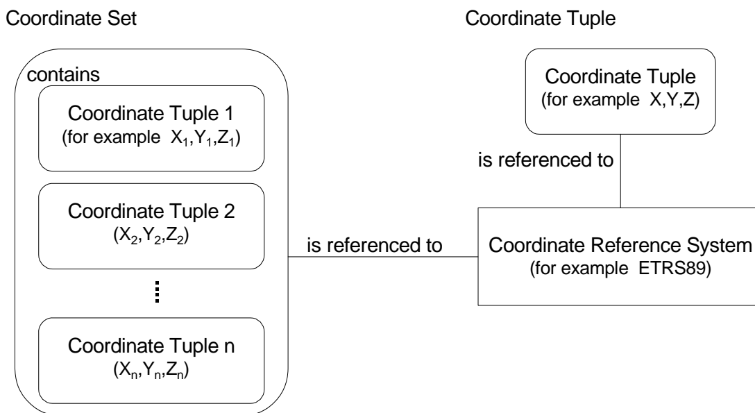
Figure 1 — Conceptual relationship of coordinates to a Coordinate Reference System (CRS)
