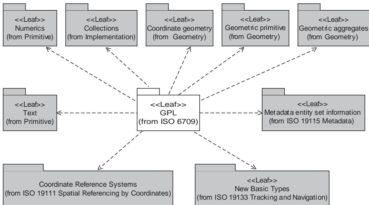
Figure C.2 — UML package dependencies
