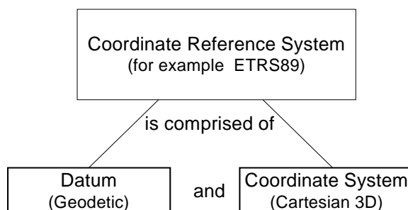
Figure 2 — Conceptual Model of a Coordinate Reference System
