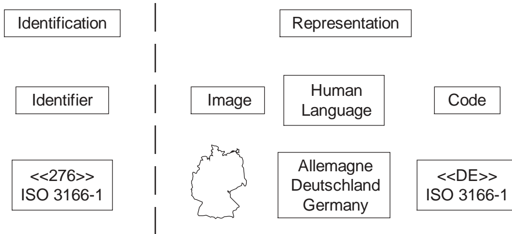
Figure 6 — Example of the distinction between identifiers used in an information technology interface and representations used in a user interface
