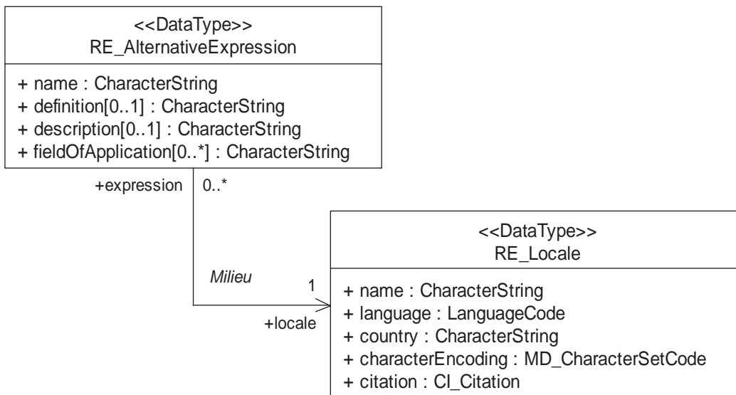
Figure 18 — RE_AlternativeExpression and RE_Locale
